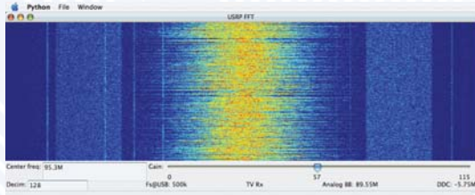
Spectrogram of an FM transmitter with IBOC sidebands. GNU Radio and USRP running on Mac OS X.
